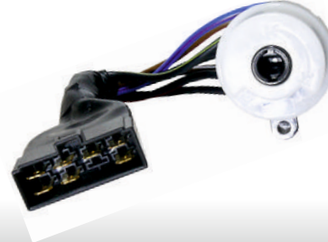
KA 1298 TOYOTA COROLLA AE80 1985->1989 OEM NO : 8445020220
