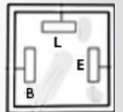
VF 1010 12VOLT 3PİN FLASER ISUZU NKR / ISUZU WIDE / ISUZU RODEO / UNIVERSAL JAPON ARAÇLARI İÇİN OEM NO : 0665004100 / RH257EL
