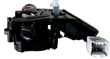
VALOR 0325 : HONDA ACCORD / HONDA CRV BAGAJ KİLİT MOTORU 1998-2003 5 PİN OEM NO : 74851S84A01
