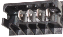
AN 0580 RENAULT MEGANE ARKA CAM REZİSTANS ANAHTARI OEM NO : 7700841243
