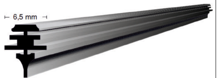
RLT 15 SLT 385 mm RLT 16 SLT 400 mm RLT 18 SLT 450 mm RLT 20 SLT 500 mm RLT 22 SLT 550 mm RLT 24 600 mm RLT 29 SLT 6,5 x 700 mm TELLİ SIRTİ KALIN LASTİK
